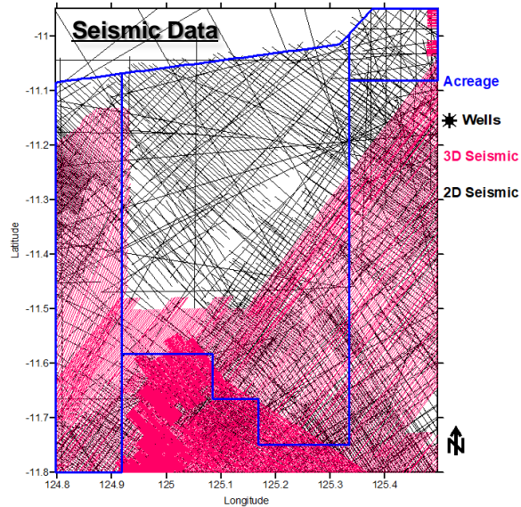
Vulcan Sub-Basin, AC20-2: Acreage Boundary, Wells and 2D & 3D Seismic
