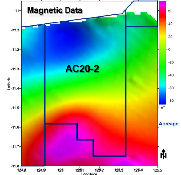
Vulcan Sub-Basin, AC20-2: Acreage Boundaries, Wells and Magnetic Data
