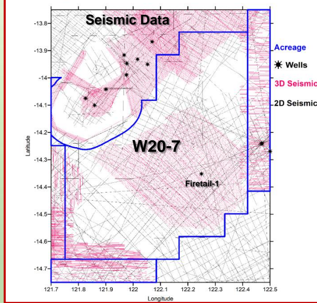
Browse Basin, W20-7: Acreage Boundary, Wells and 2D & 3D Seismic
