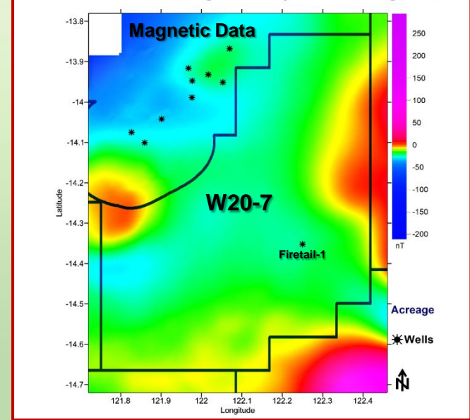
Browse Basin, W20-7: Acreage Boundary, Wells and Magnetic Data
